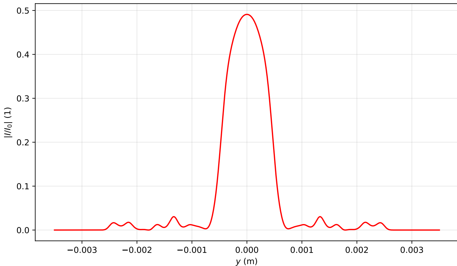
Intensity profile I(x=0, y, z=2.866)/I_0 , P_{in}=3.5P_{cr} , artificial time
